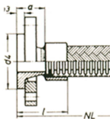
Flange connection, swivelling
