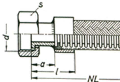
Pipe fitting
