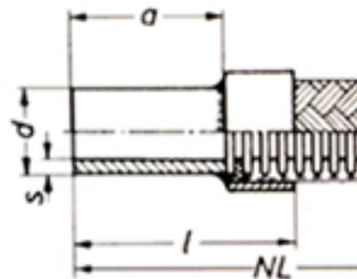
Pipe fitting
