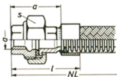
Threaded fitting, internal thread
